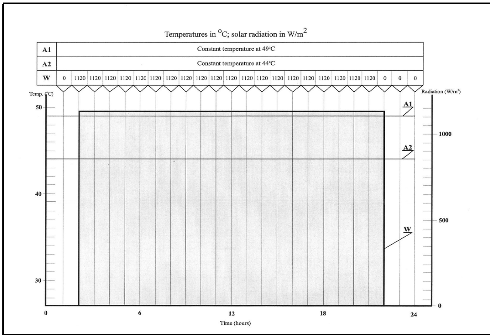
Figure 505.6-2. Procedure II – Steady state test.
