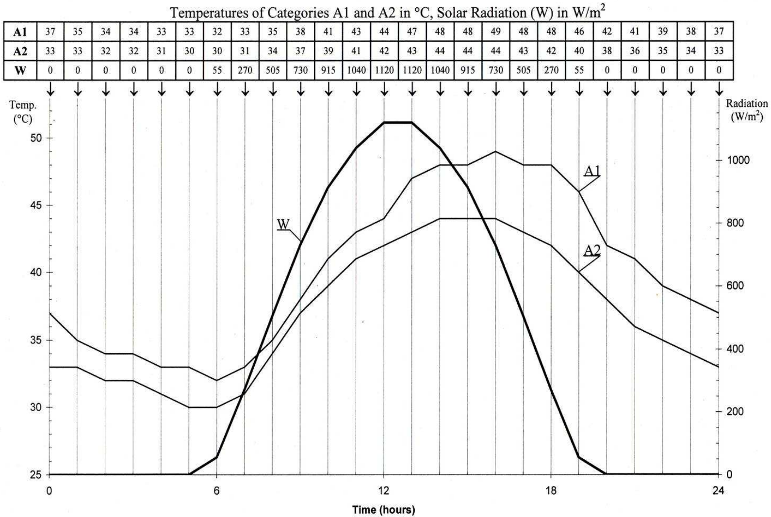
Figure 505.6-1. Procedure I – Cycling test.
