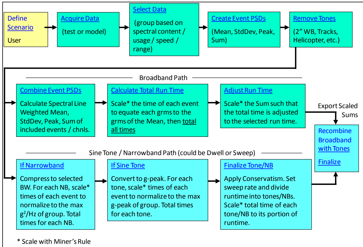
Figure 514.7F-D.1. VSD flowchart.
