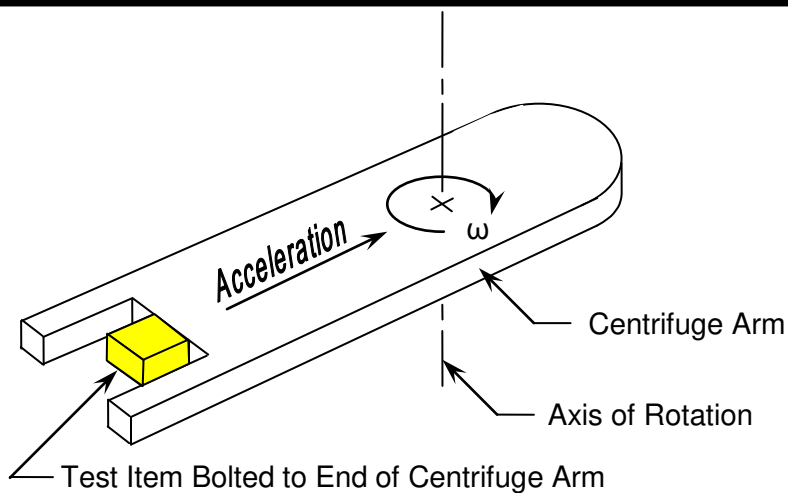
Typical Installation
