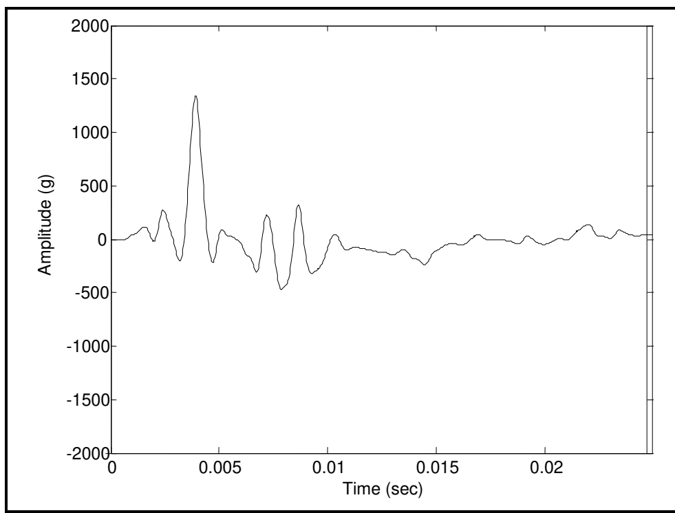
Figure 519.7C-4b. Sample RMP model random components r(t) , (single pulse).
