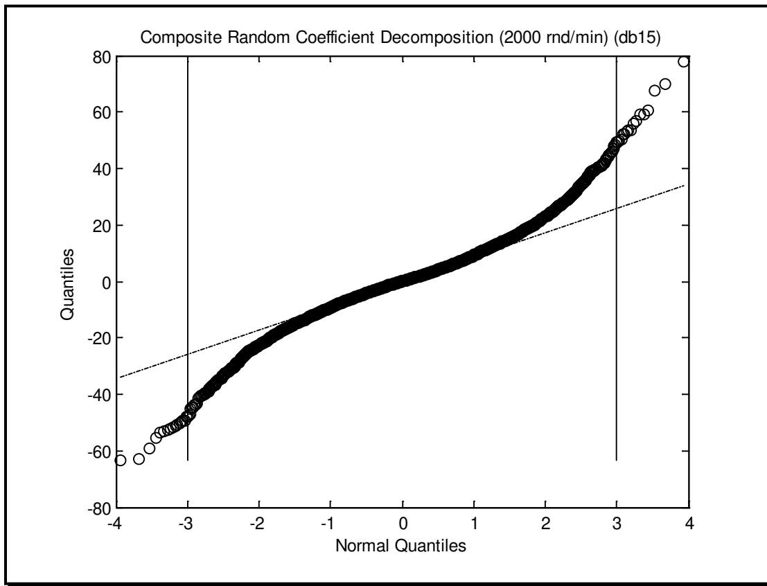
Figure 519.7B-7a. qq-Plot for composite random component decomposition, 2000 rmd/min.
