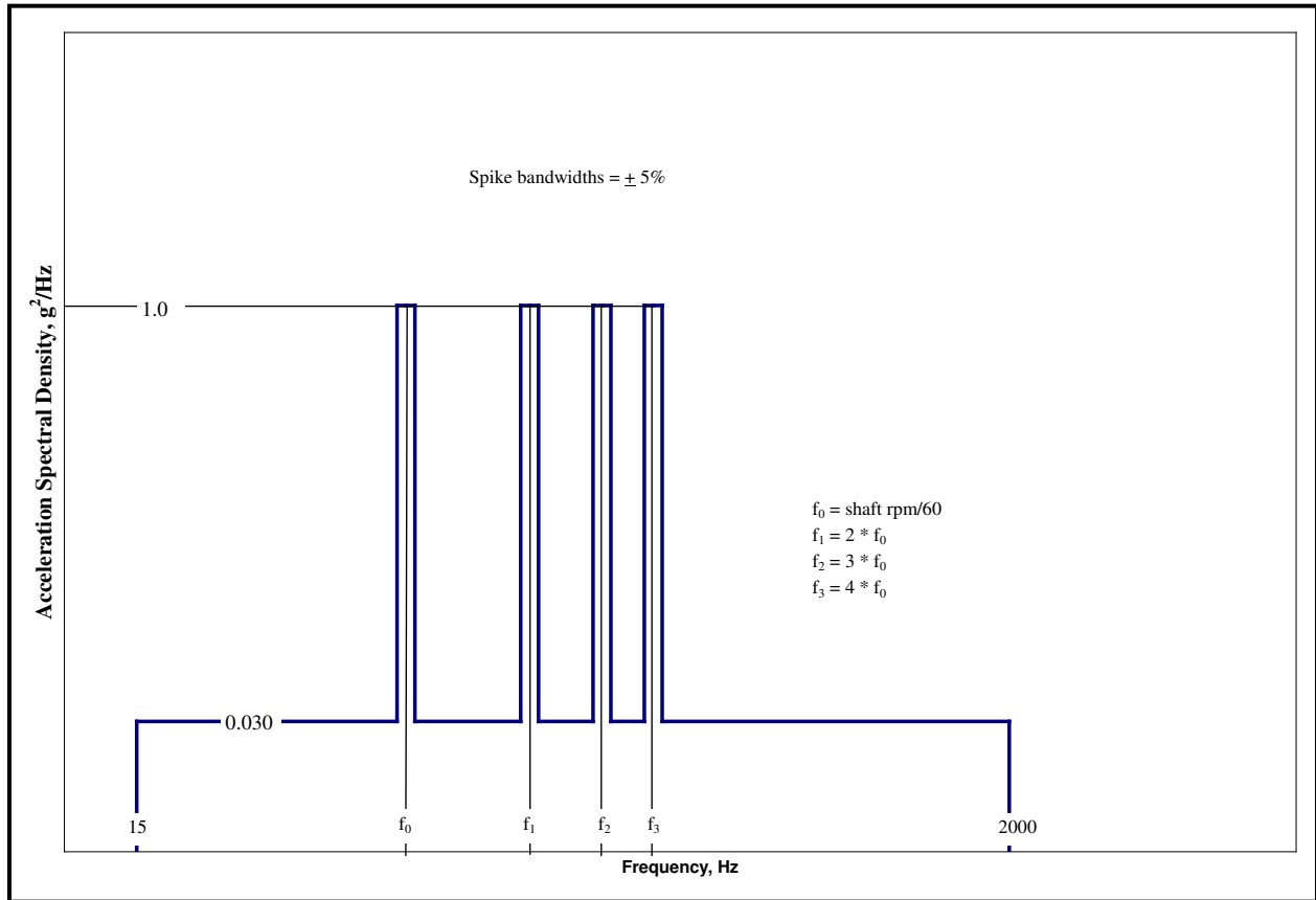
Figure 514.7D-10. Category 22 - Turbine engine vibration exposure.
