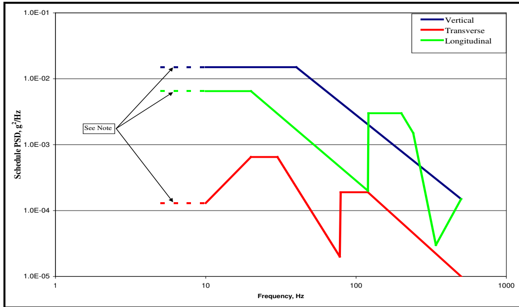
Figure 514.7C-2 – Category 4 – Common carrier (US highway truck vibration exposure).
