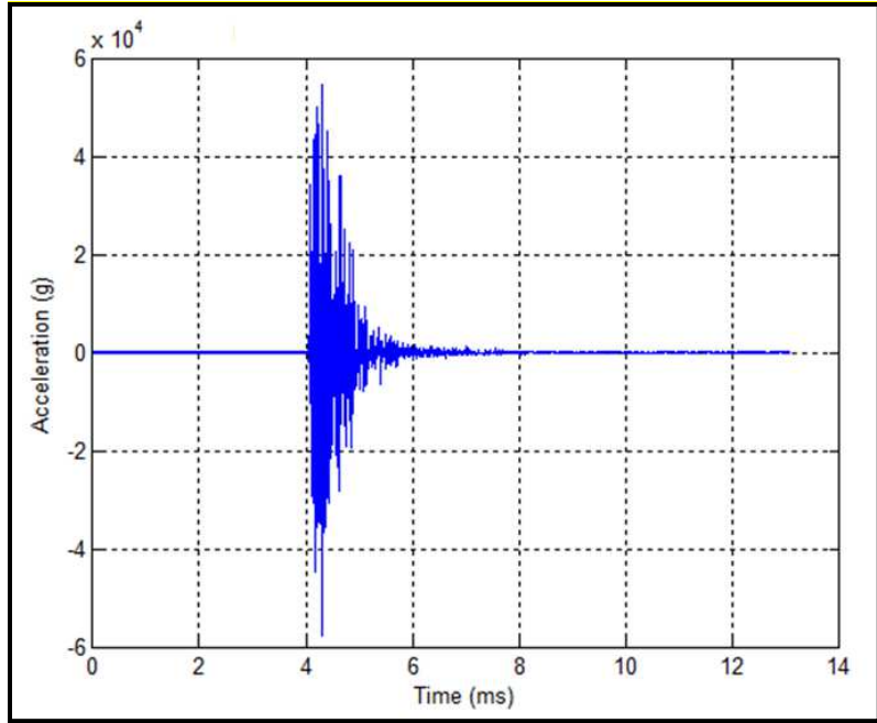
Figure 517.2-3. Full duration near-field, accelerometer pyroshock time history.
