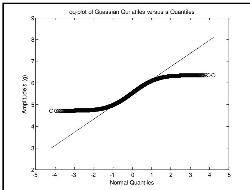
Figure 525.1A-12. Transient vibration q-q plot for s versus Gaussian.
