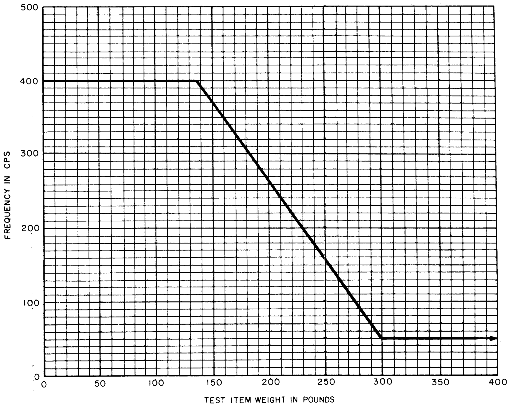
Figure 514-7. Weight vs. frequency. Equipment installed in ground vehicles.
