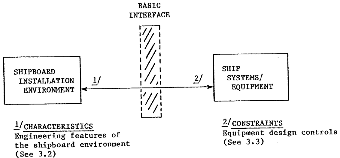
FIGURE 1. Interface .
