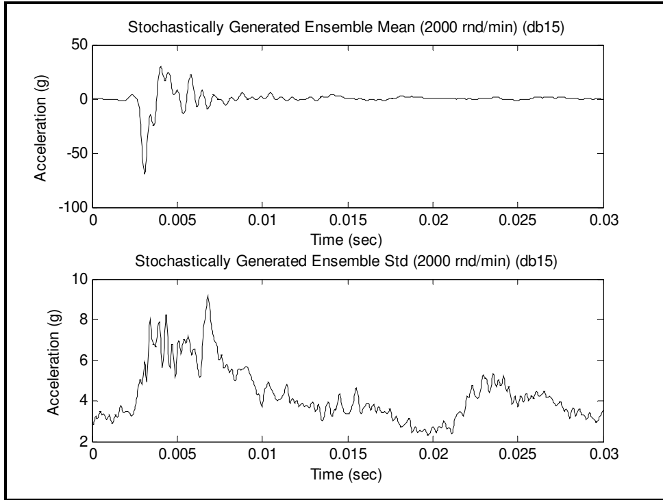
Figure 519.6B-8c. Ensemble and stochastically generated pulse ensemble random component standard deviation (2000 rpd/min).
