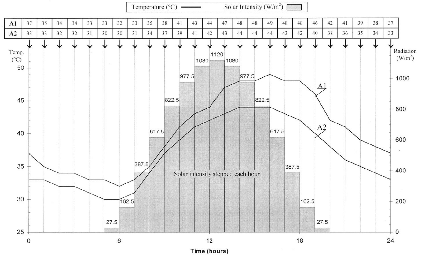
Figure 505.5C-5. Method for conducting Procedure I with solar radiation controlled in one-hour steps.
