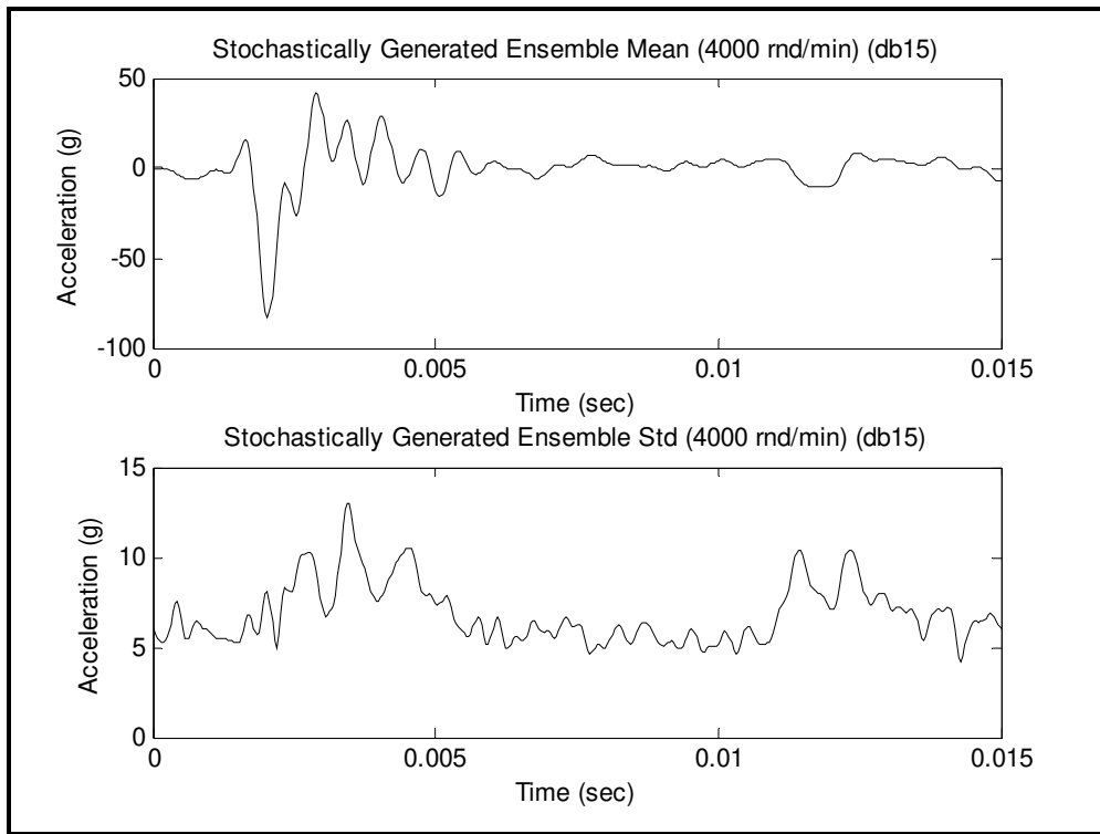
Figure 519.6B-8d. Ensemble and stochastically generated pulse ensemble random component standard deviation (4000 rpd/min)
