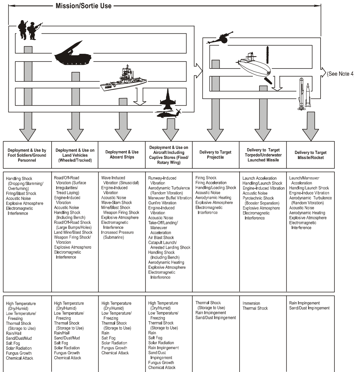
FIGURE 1-4b. Generalized life cycle histories for military hardware.
