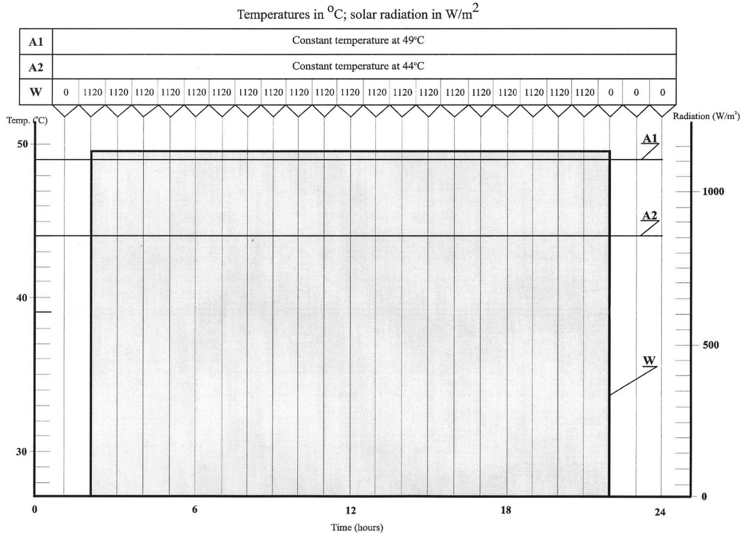
FIGURE 505.5-2. Procedure 2 - Steady State Test.
