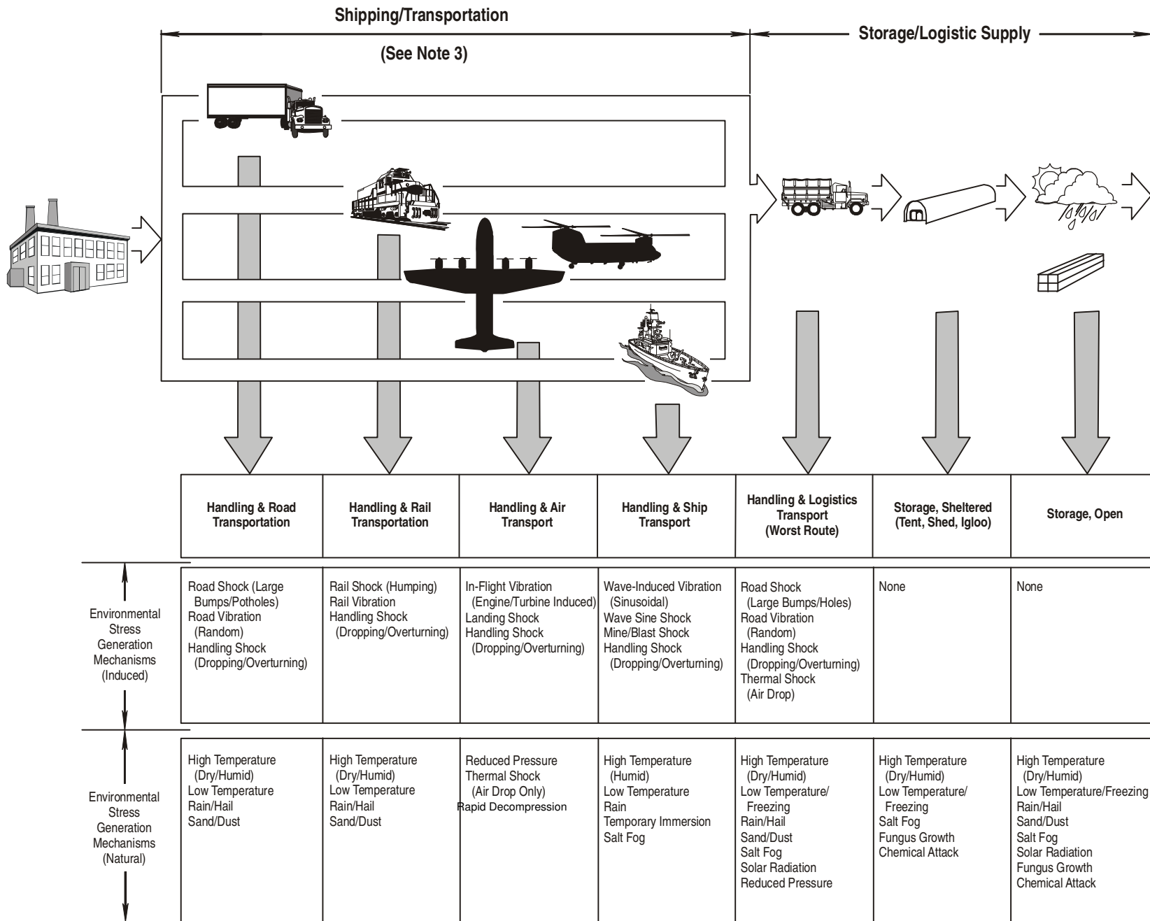
FIGURE 1-4a. Generalized life cycle histories for military hardware.
