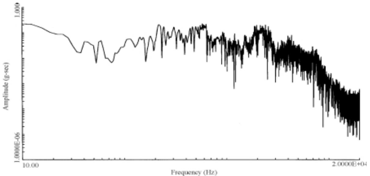
FIGURE 516.5-7. Sample shock response acceleration FS estimate.
