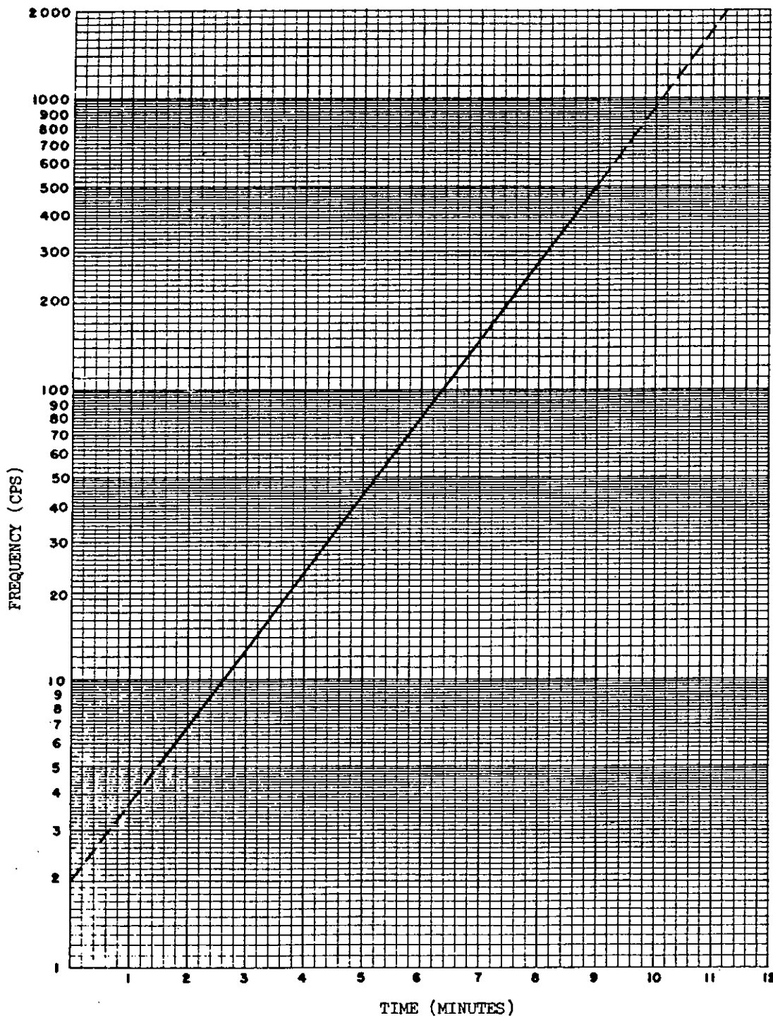
FIGURE 514-8. Logarithmic cycling rates: For cycling tcs's of less than 500 cps maximum frequency, the frequency range shall be cycled logarithmically from 5 cps to maximum in 7.5 minutes for the total cycling time specified.
