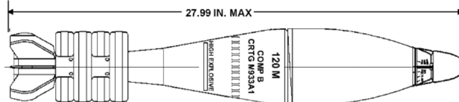
Figure 1. Cartridge, 120mm: IIE, M933A1 with Fuze, PD/DLY, M783.
